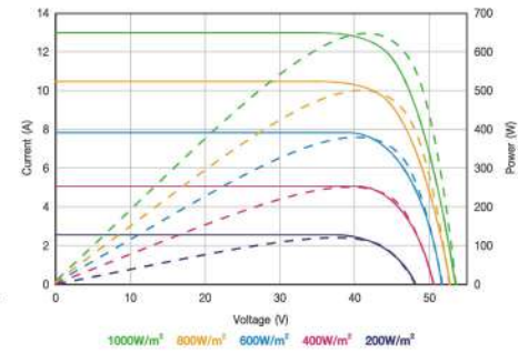
P-V curve at different Irradiation 680w
